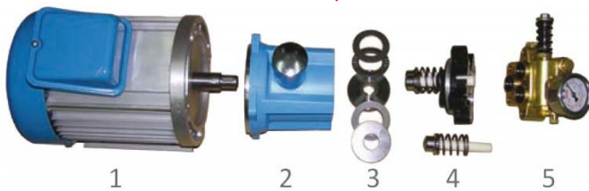
1/2HP, 1/3HP Pump break down
